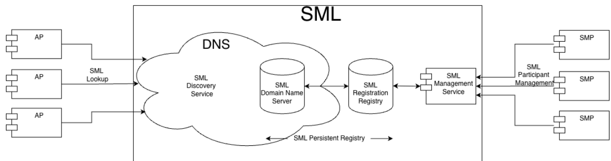
The SML interface connections to the Peppol Network
