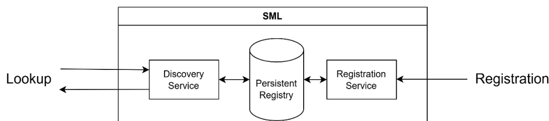
The Interfaces of the SML
